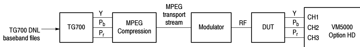
Figure F-1: Using TG700 baseband test signals
