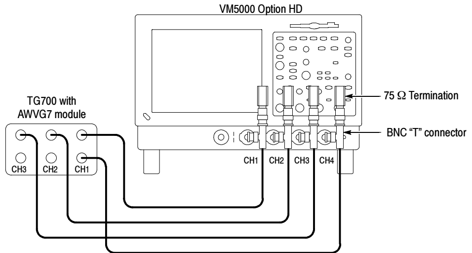
Figure B-3: Frequency accuracy test hookup
